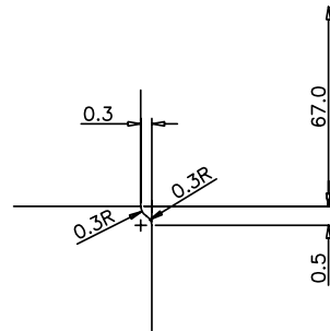
PANEL DETAIL SCALE 10:1
